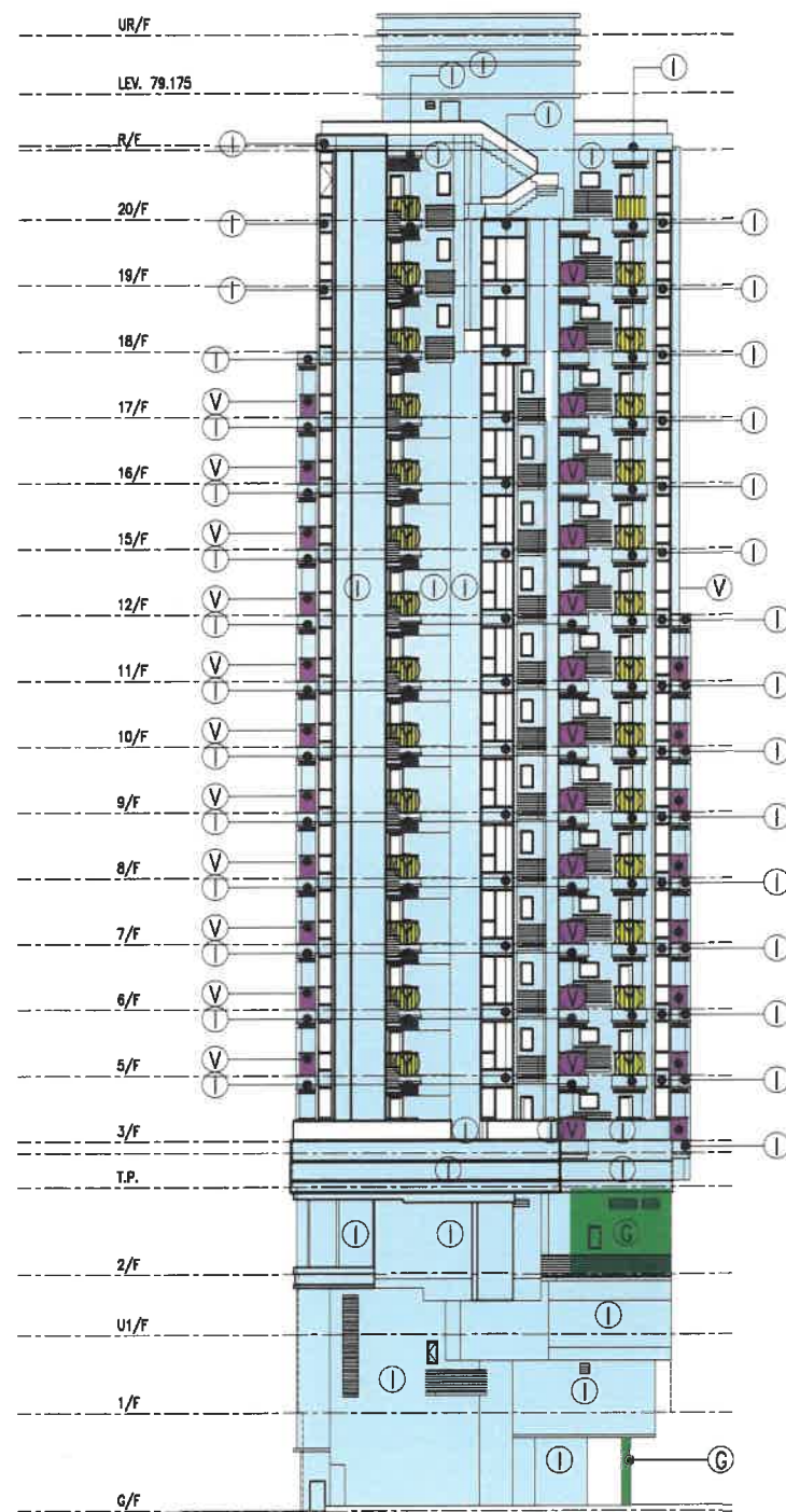
WEST ELEVATION (4/F, 13/F & 14/F FLOOR NUMBERING OMITTED) 'FOR IDENTIFICATION PURPOSE ONLY'
