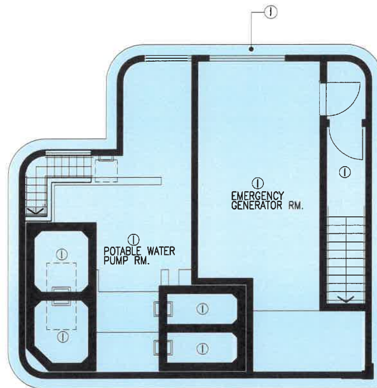
LEVEL 79.175 FLOOR PLAN 'FOR IDENTIFICATION PURPOSE ONLY'
