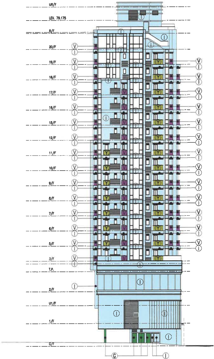
EAST ELEVATION (4/F, 13/F & 14/F FLOOR NUMBERING OMITTED) 'FOR IDENTIFICATION PURPOSE ONLY'
