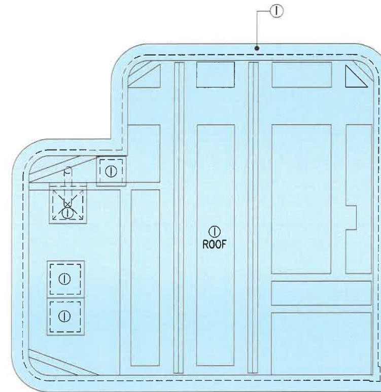
UPPER ROOF FLOOR PLAN 'FOR IDENTIFICATION PURPOSE ONLY'
